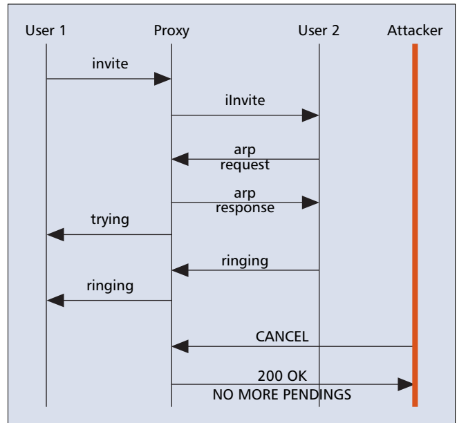
■ Figure 12. CANCEL attack.
