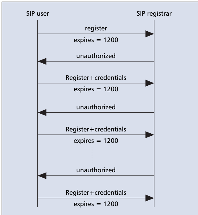
■ Figure 5. Attack against SIP registrar server.
