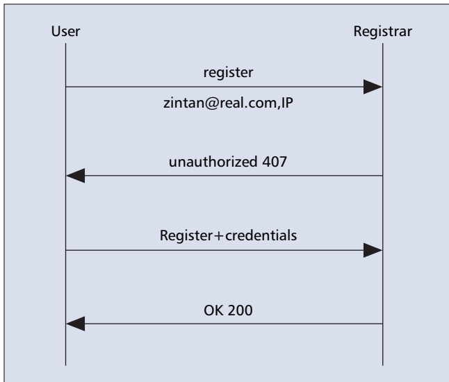
■ Figure 1. Registration procedure.
