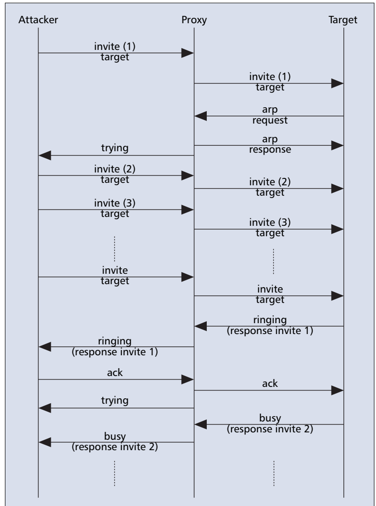
■ Figure 7. Alternative flooding INVITE scenario.
