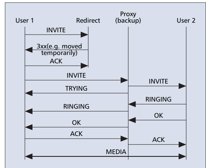
■ Figure 3. SIP Call utilizing a Redirect proxy.
