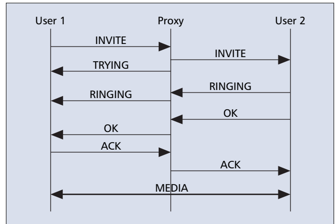
■ Figure 2. Calling a user in SIP.
