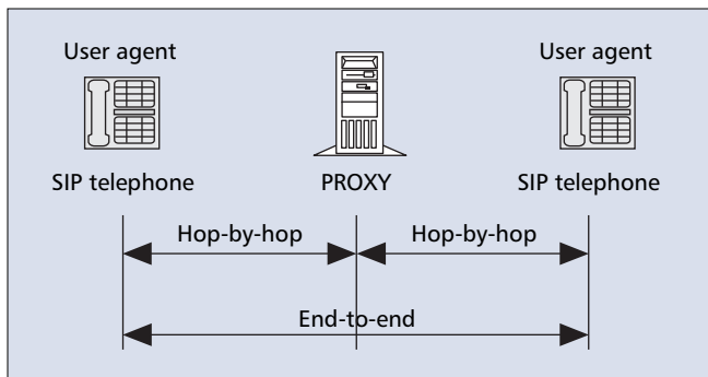
■ Figure 4. SIP security mechanisms.
