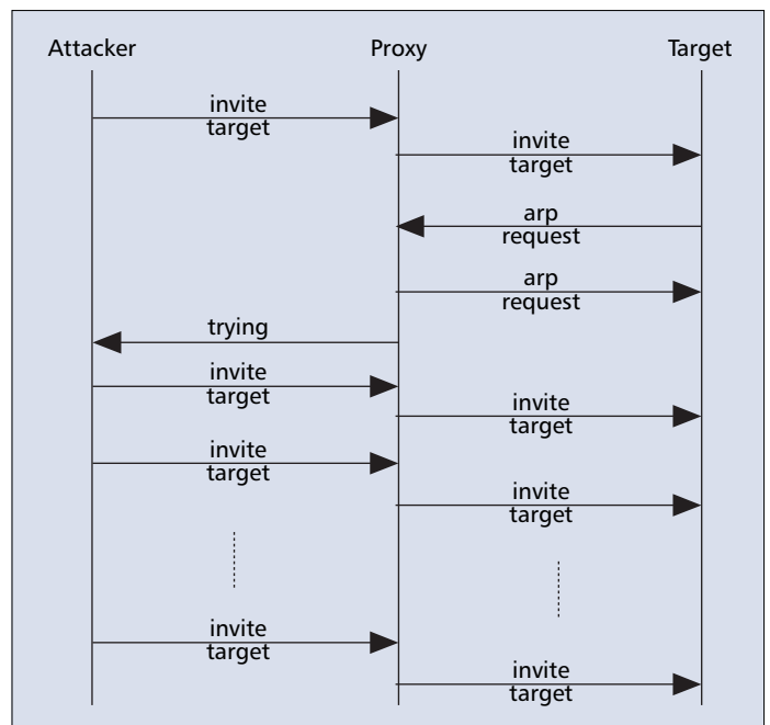
■ Figure 6. Flood with INVITE messages.
