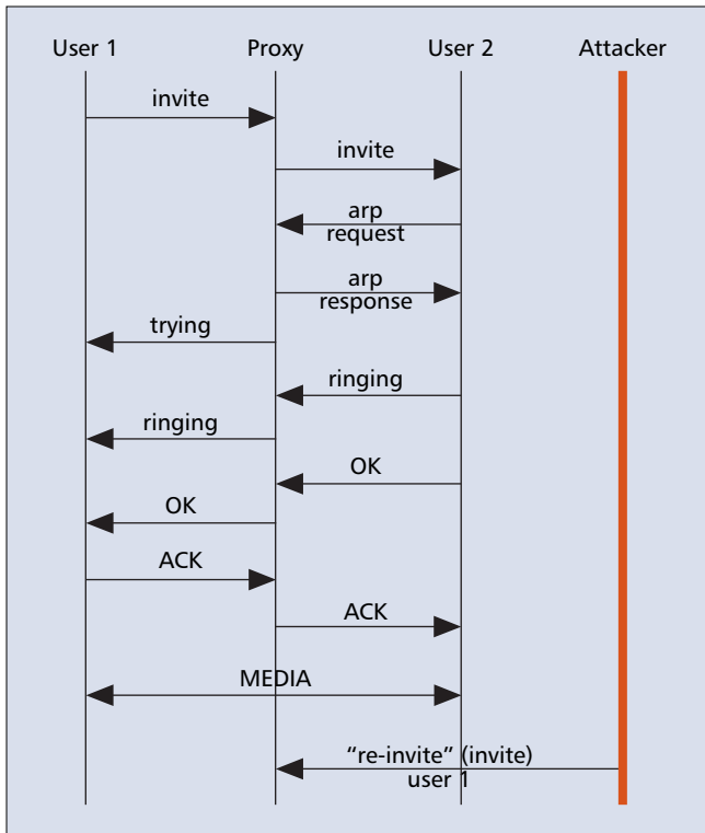
■ Figure 13. "Re-INVITE" attack.
