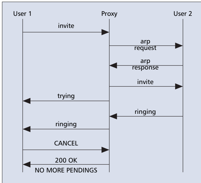
■ Figure 11. CANCEL request.
