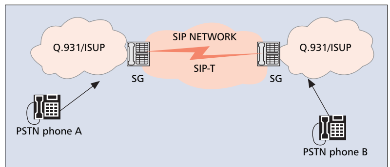
■ Figure 15. PSTN and SIP Interconnection.
