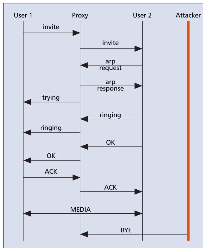
■ Figure 10. BYE attack.
