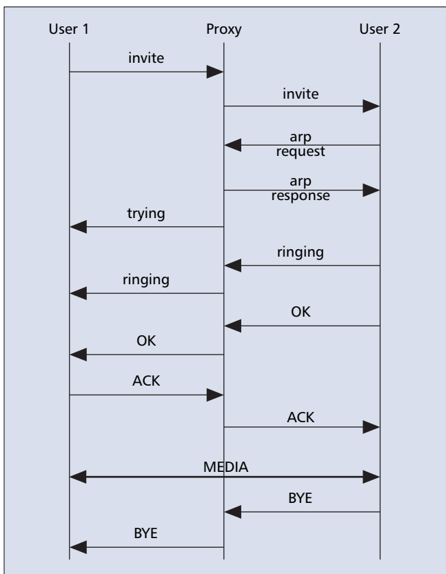
■ Figure 9. Normal session termination.
